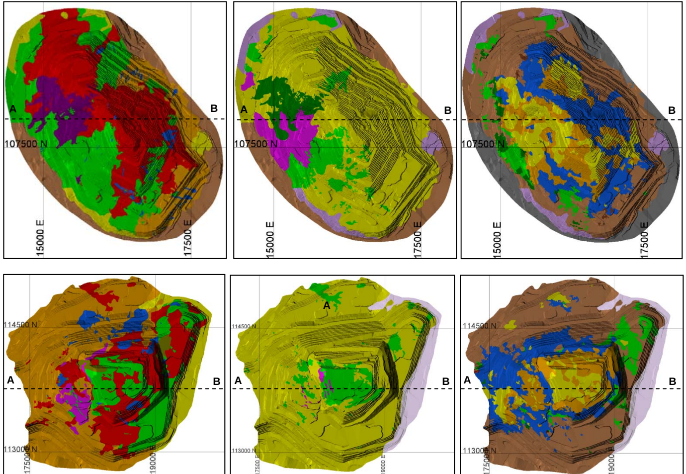
Figure 2: Mine geological setting for Escondida (upper row) and Escondida Norte (lower row) of lithology (left column), alteration (middle column) and mineral zones (right column). Dashed lines shows location of sections. See Figure 3 for explanation of geological units.
